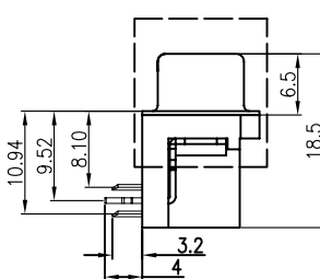
WITH SCREW AND RIVET TYPE
