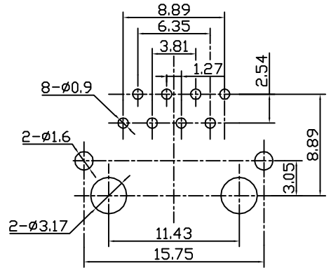
PCB LAYOUT COMPONENT SIDE TOLERANCES ±0.05 Thickness=1.6mm
