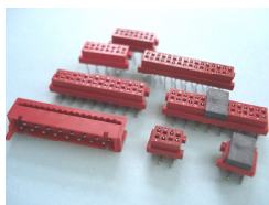
DS3900 series Mini connector red, pitch 1.27 mm. (flatcable-to-board connector series)
